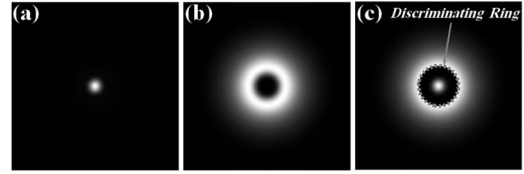
FIG. 3. Calculated far-field patterns of OAM modes m=0 and m=4 generated by the QP for input OAM m = \pm 2 [the input beam was assumed to HyGG -2,±2 ( r, \phi, 0, 1 ) (Ref. 18) mode]. The dashed circle shows the discriminating area used in the balanced mode sorter.
